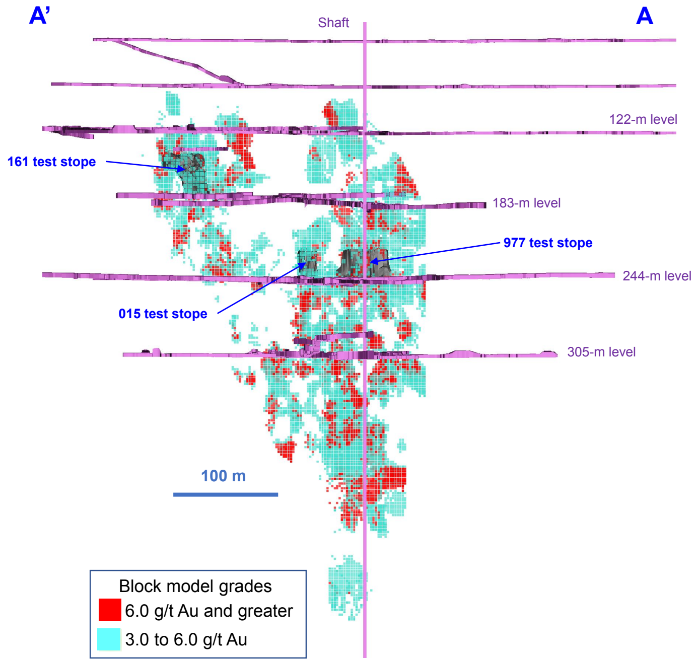
Diagram 3: 2018 Mineral Resource Estimate at 3.0 g/t Au Cut-off Grade, Zone 1 – Block Model Grade Distribution – Section View Looking East (mine grid)
