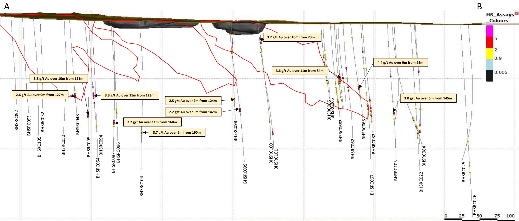
Figure 3 – Long Section with Highlighted Intersections
