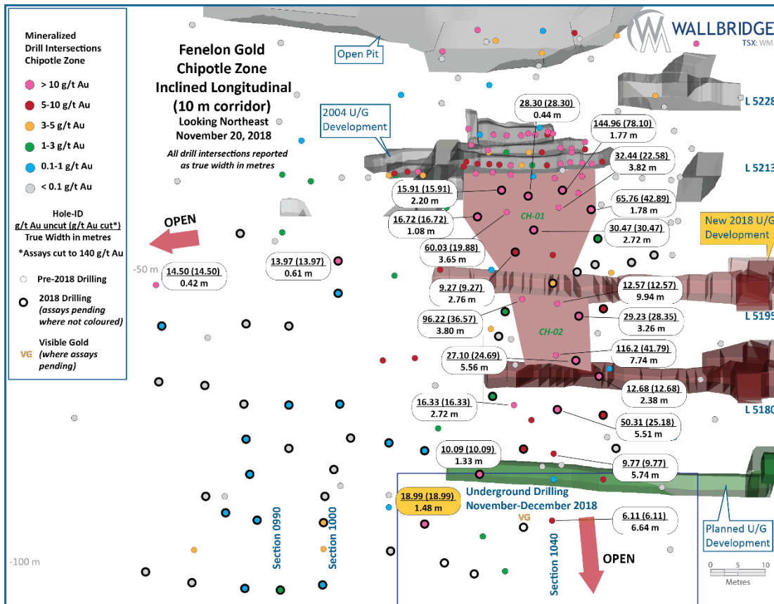
Figure 6: Fenelon Gold, Chipotle Zone Longitudinal
