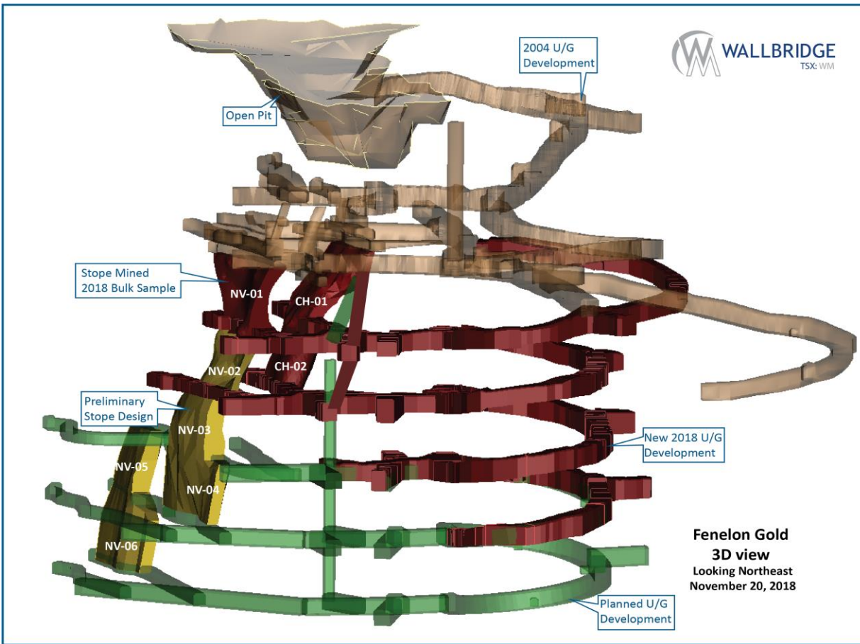
Figure 3: Fenelon Gold, 3D View
