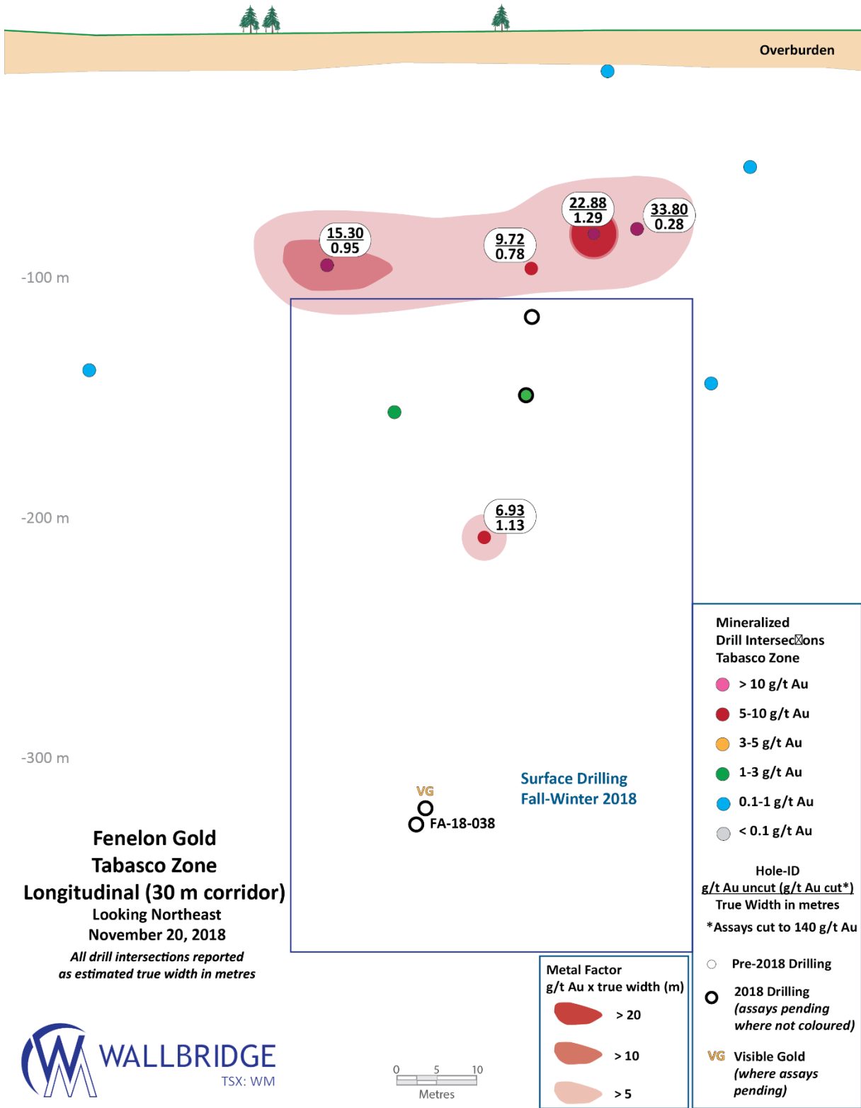
Figure 7: Fenelon Gold, Tabasco Zone Longitudinal
