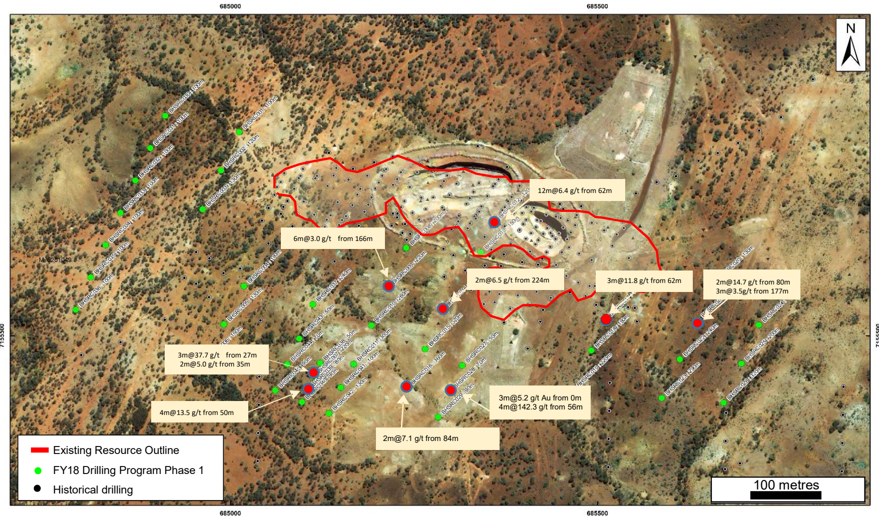
Figure 2 – Hermes South Plan View of Phase 1 RC Drilling
