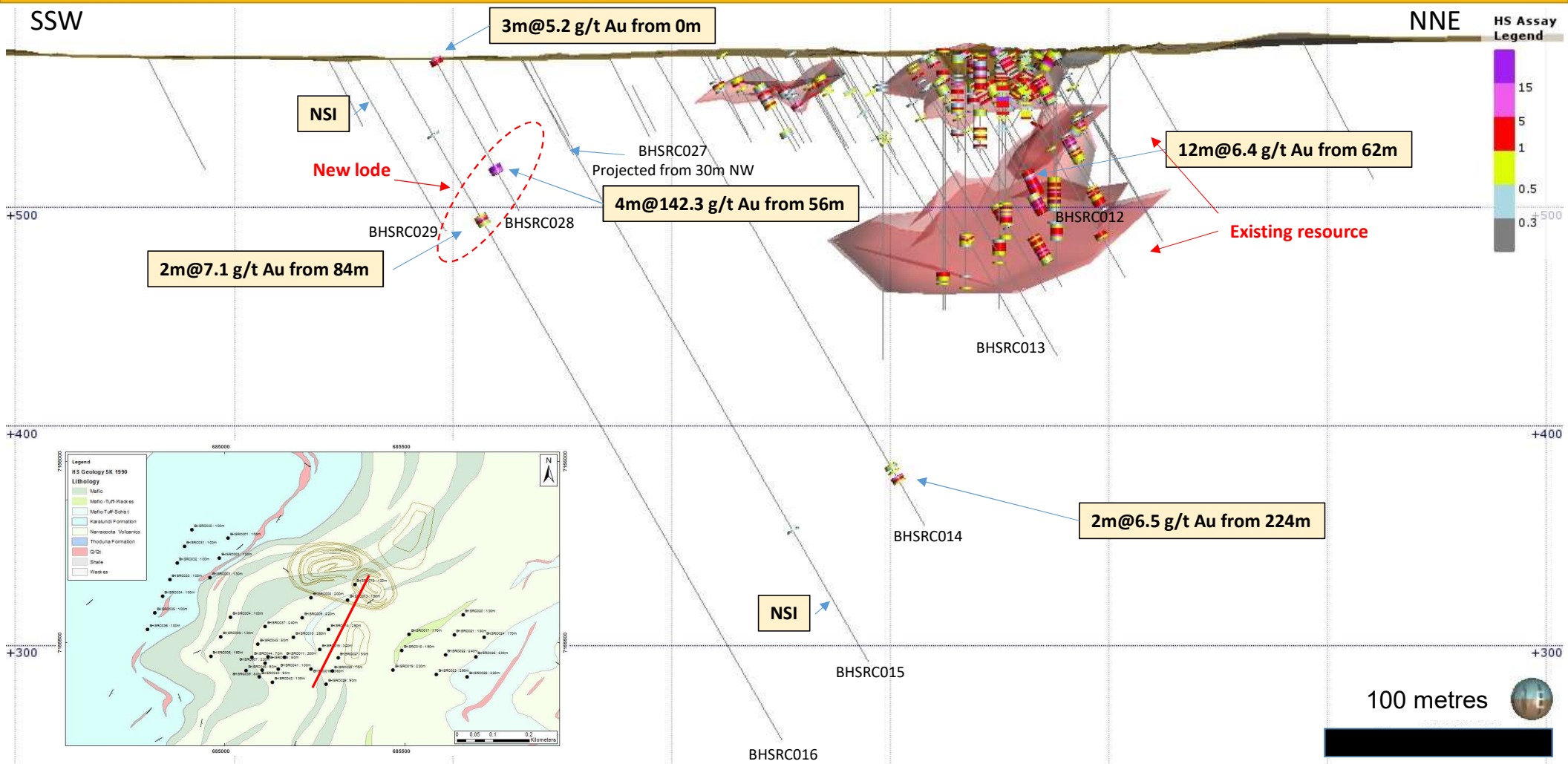
Figure 4 – Hermes South - Cross Section #2
