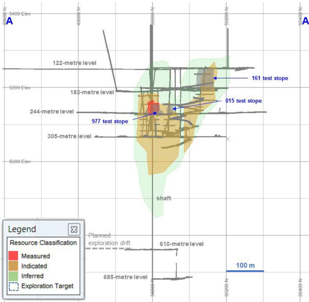
Diagram 2: 2018 Mineral Resource Block Model Diagram Zone 1 (F2 Basalt) – Section View Looking West (Mine-Grid)
