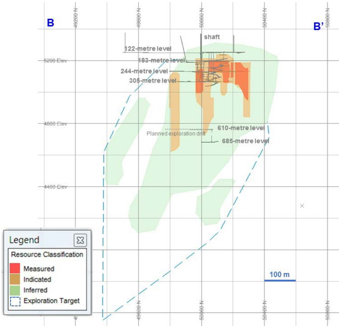
Diagram 3: 2018 Mineral Resource Block Model Diagram Zone 2 (Hanging Wall and West Limb Basalts) – Section View Looking West (Mine-Grid)
