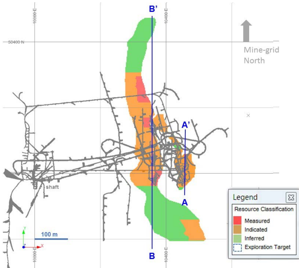
Diagram 1: 2018 Mineral Resource Block Model Diagram – Plan View, 305-Metre Level
