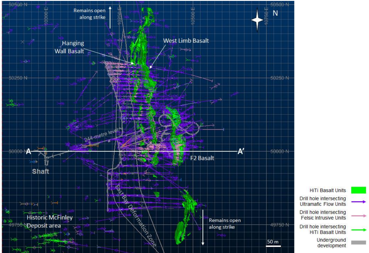
Diagram 1: Preliminary Structural Interpretation (2018) of the F2 Gold Deposit – Plan View of the 244-metre level
