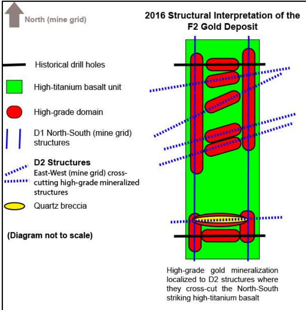
Diagram 4: Conceptual 2016 Structural Interpretation - Plan View
