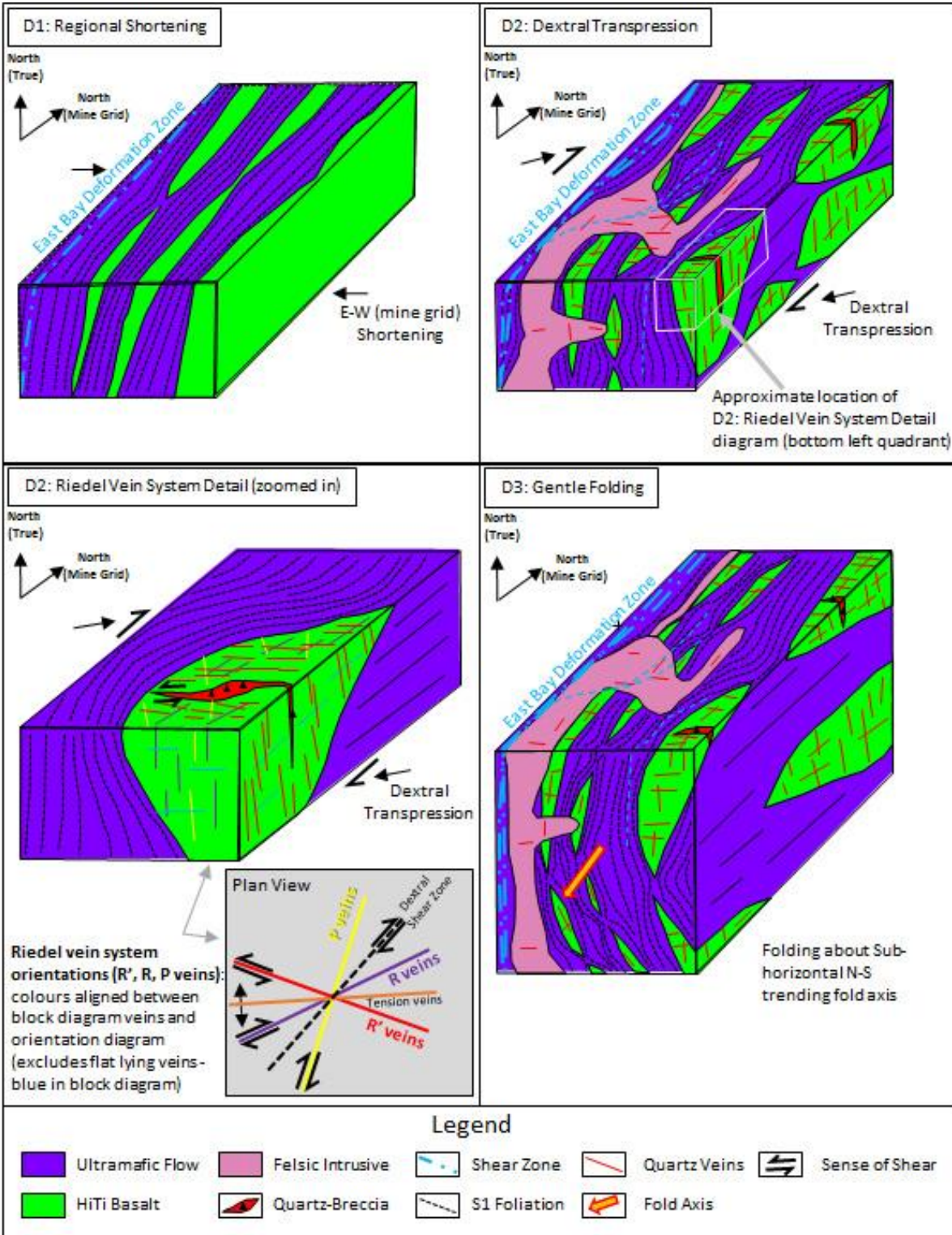
Diagram 3: Preliminary Structural Interpretation (2018) of the F2 Gold Deposit – Conceptual Summary the Deformation and Structural Controls on the Gold Mineralization – Isometric Views (diagram not to scale)
