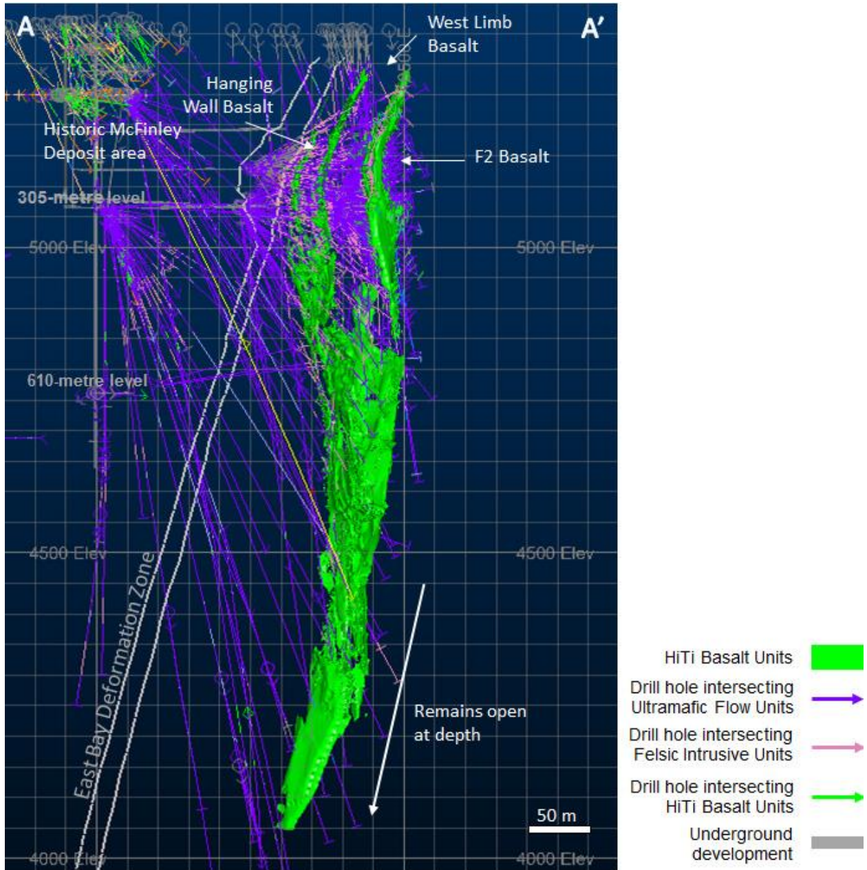
Diagram 2: Preliminary Structural Interpretation (2018) of the F2 Gold Deposit – Section View A to A'
