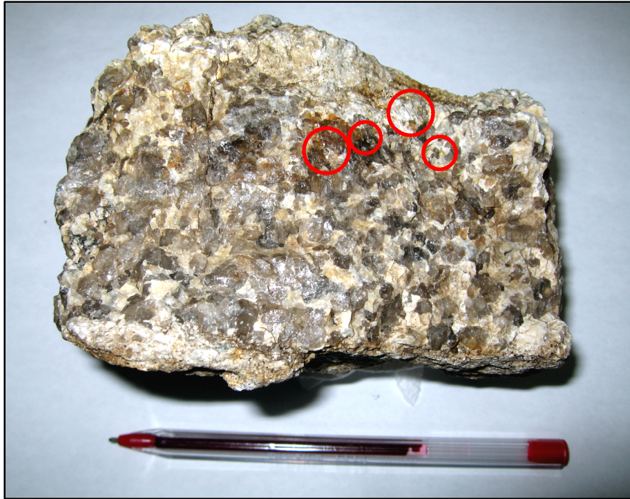
Trench Prospect : 1,500 g/t Au in quartz-feldspar pegmatite (Sample S657741)
