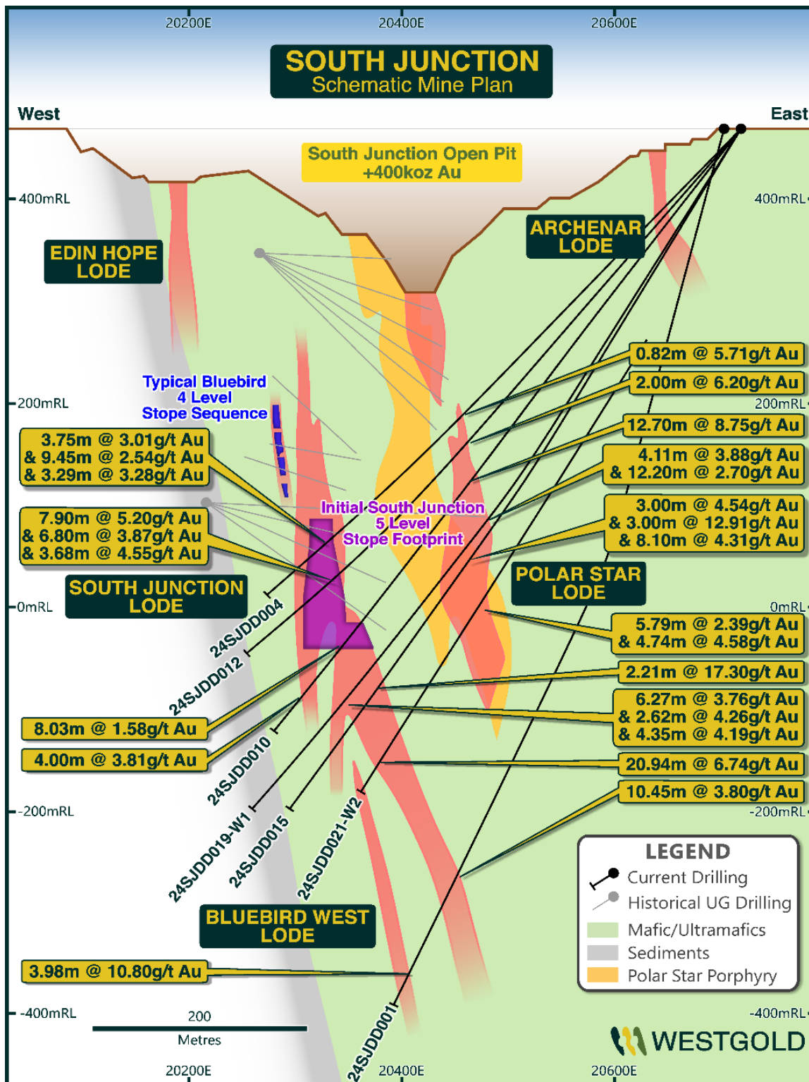
Figure 3 – South Junction schematic mine layout showing the scale of a typical South Junction stoping panel as compared to a typical stoping panel of the Bluebird mine (Refer Appendix B for detailed drill results).
