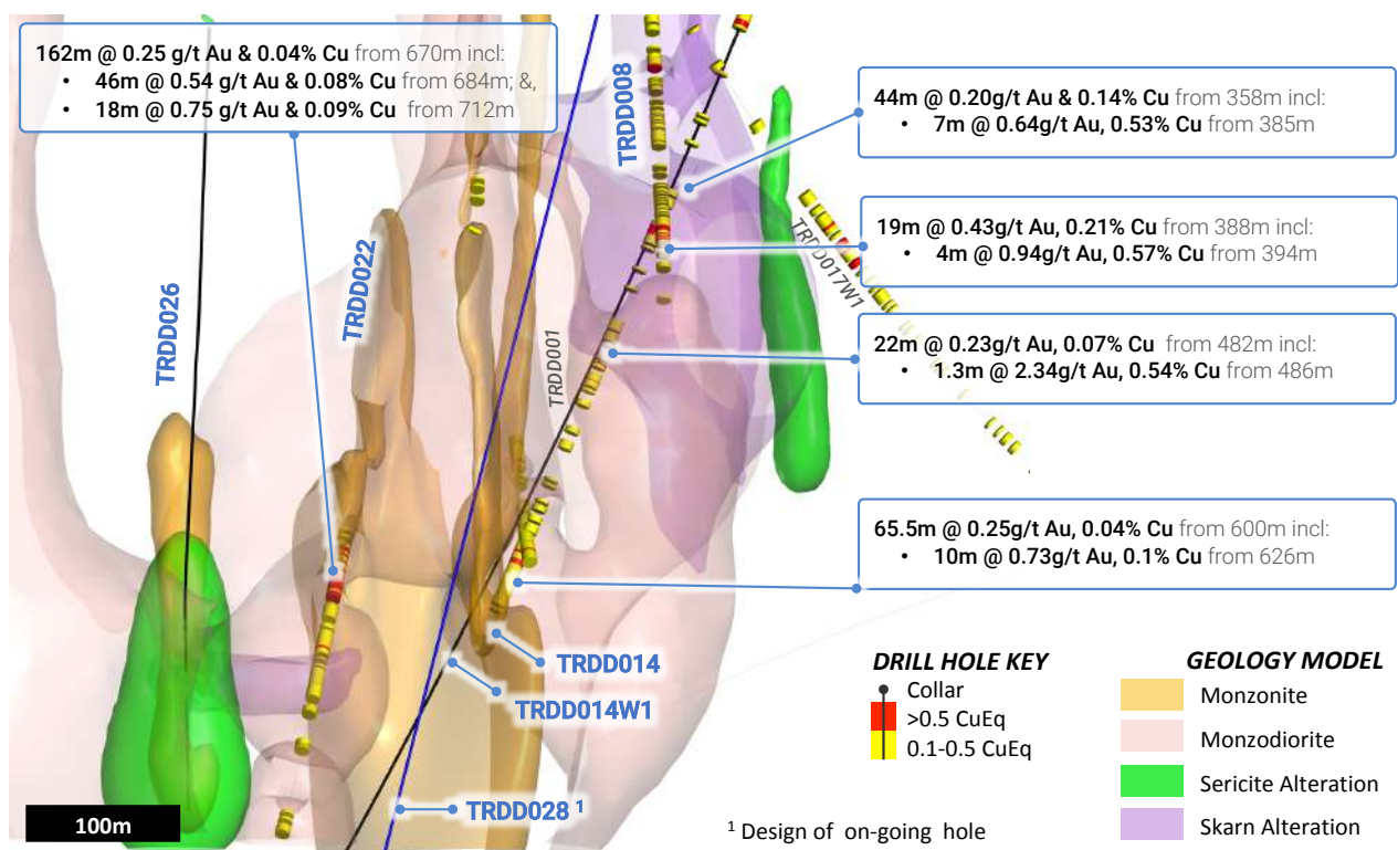
(c) Insert with mineralised intervals and illustration of strike/down dip target of TRDDo28, noting the distance from TRDDo28 to TRDDo14W1 is approximately 100m west and 115m south-west to TRDDo22
