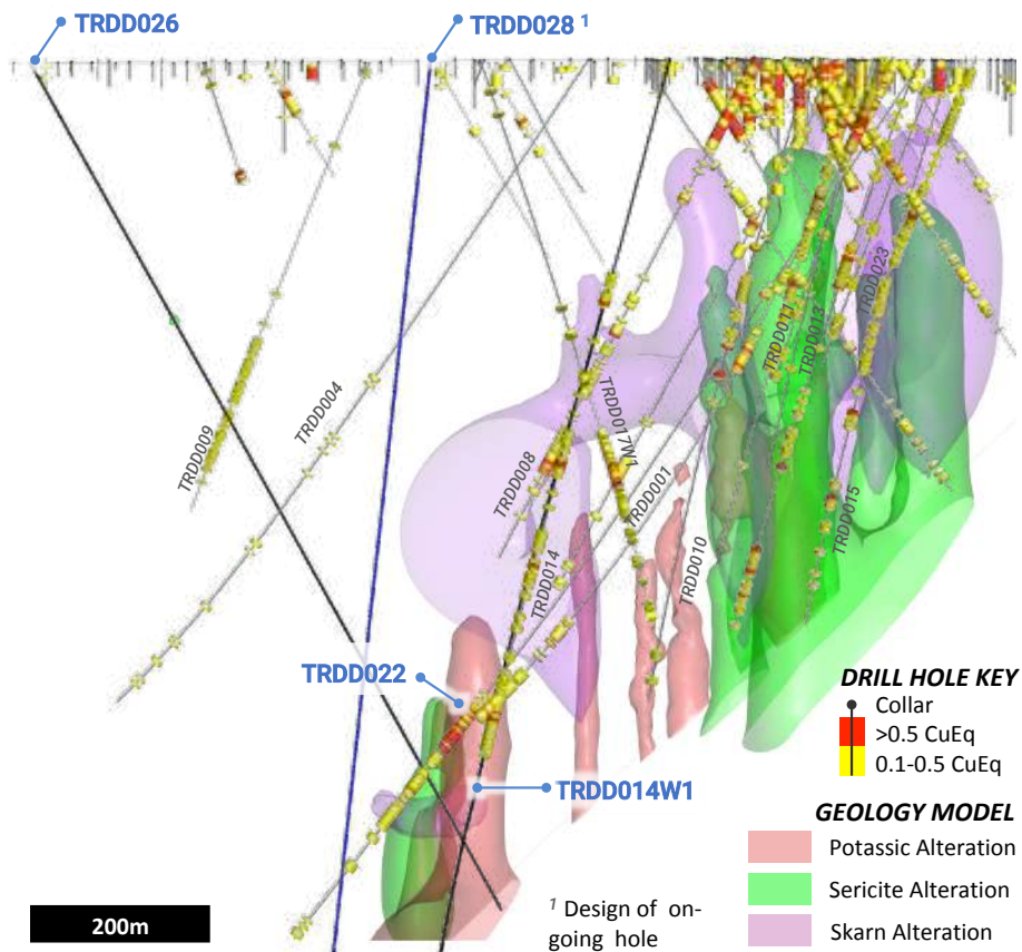
(c) Insert with mineralised intervals and illustration of strike/down dip target of TRDDo28, noting the distance from TRDDo28 to TRDDo14W1 is approximately 100m west and 115m south-west to TRDDo22
