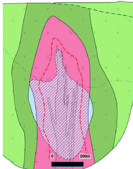
Figure 4: The clusters of deposits at the neighbouring Northparkes mine and at Cadia-Ridgeway exhibit multiple intrusive systems and an alteration, lithology and mineralised setting not dissimilar to the Trundle Park prospect around discrete mineralized cores of only hundreds of metres width that are vertically extensive
