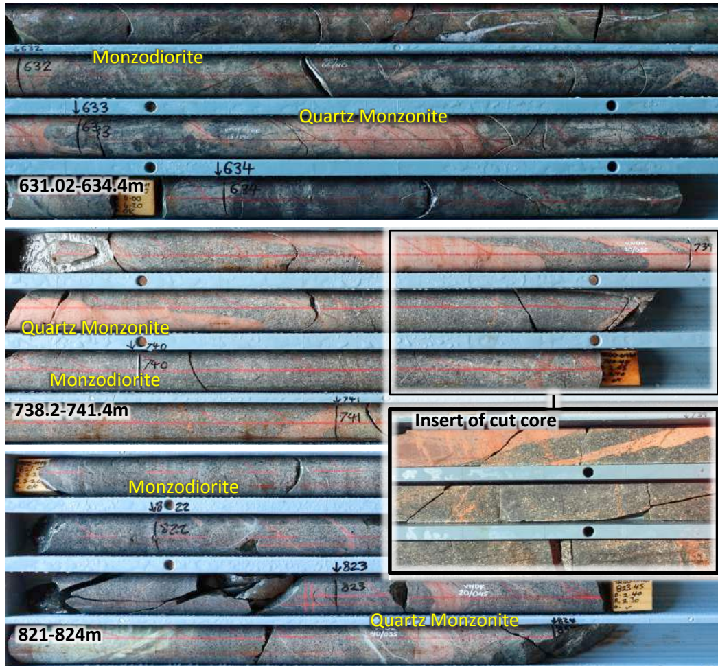
Figure 6: Examples of the rock types in hole TRDDo14W1 at the Trundle Park prospect (a) Monzonite vein-dyke system intruding a larger monzodiorite intrusion with zones of interpreted variable to strongly developed outer potassic alteration.
