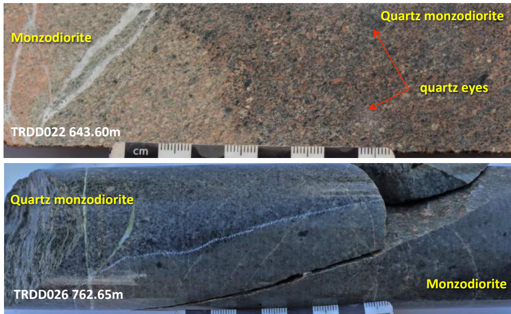
Figure 5: Examples of the rock types and multiple intrusive phases in holes TRDD022 and TRDD026 at the Trundle Park prospect
