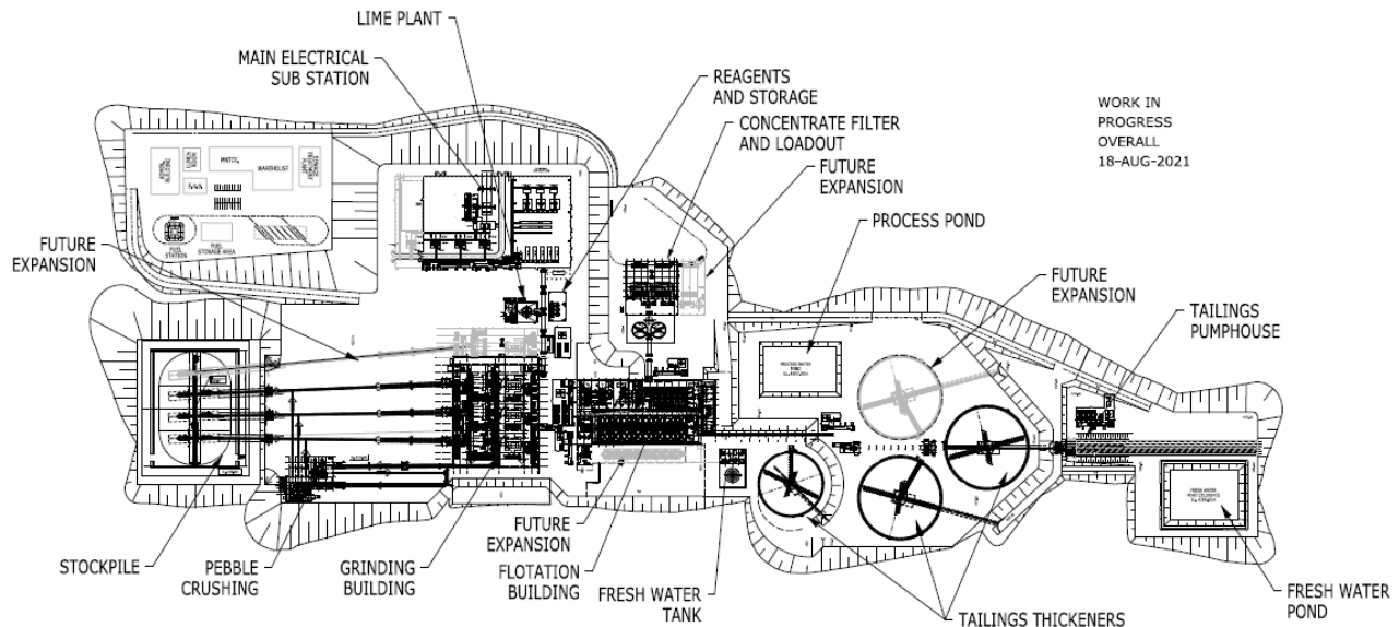
Image: Josemaria Project Revised Plant Layout, August 2021
